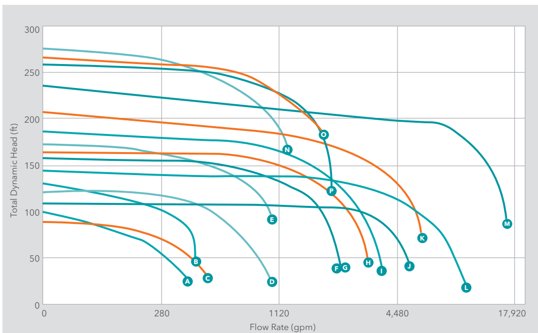
Composite curves for comparison purposes only. Consult engineering data for exact flow and head capabilities. Curves based on pumps maximum speed shown performance. May require use of VFD's for max performance.
